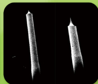
Molecular Drill
