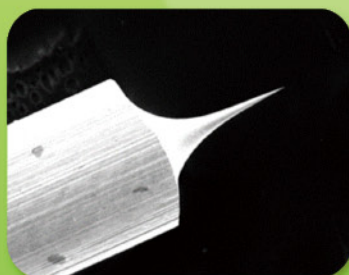
Atomic Imaging
